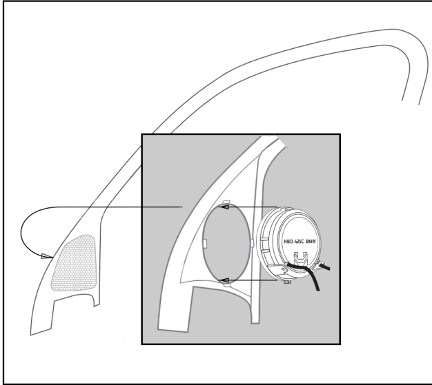
Mid-range speaker HBO-425C BMW
